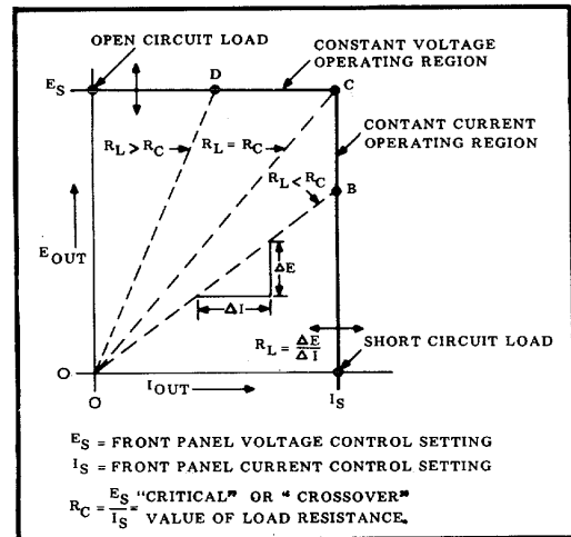
Figure 4-2. Operating Locus of a CV/CC Power Supply
