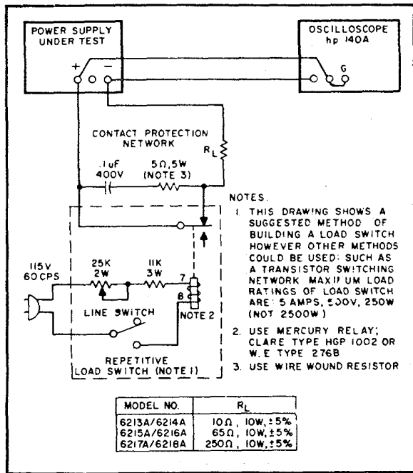
Figure 5-7. Transient Recovery Time, Test Setup
